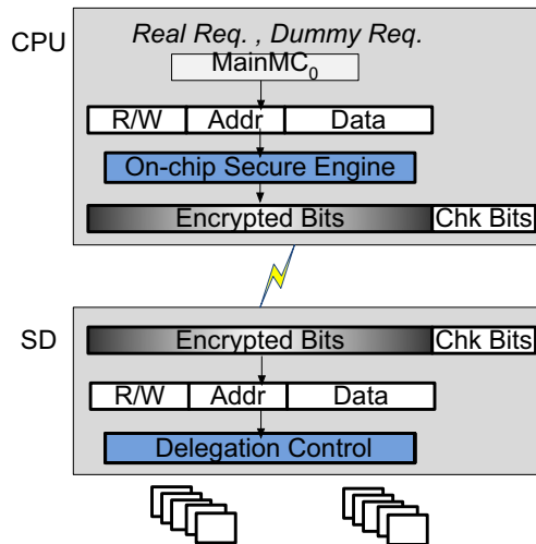
Figure 6. Delegating Path ORAM in SD.
