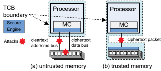
Figure 2. Comparing two TCB models.
