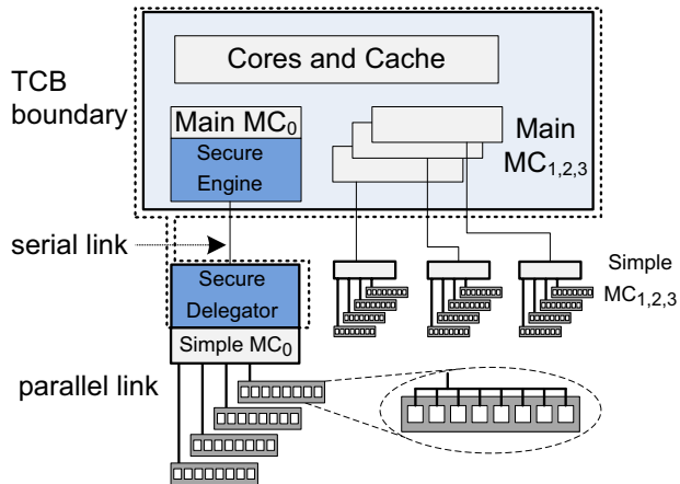
Figure 5. An overview of D-ORAM memory system.
