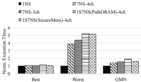
Figure 4. The performance degradation under different co-run scenarios.
