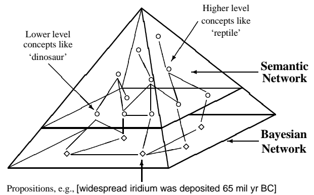
Figure 2: Sample Semantic-Bayesian Network
