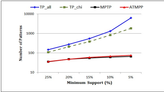
Figure 4: The number of patterns return by TP_all , TP_chi , MPTP and A-MPTP for different minimum supports.
