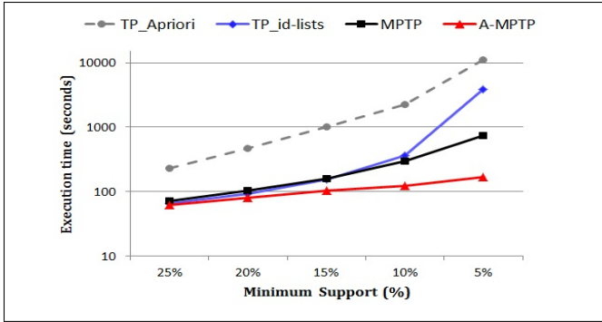
Figure 5: The running time of TP_Apriori , TP_id-lists , MPTP and A-MPTP for different minimum supports.
