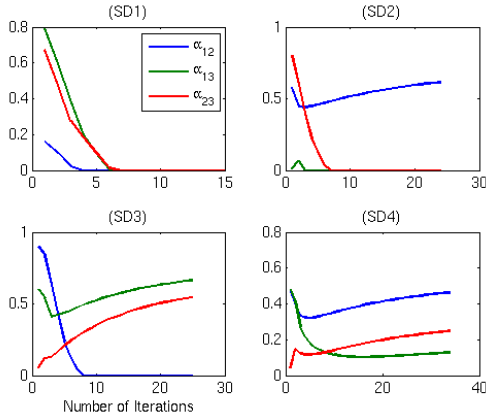
Figure 2: Profile of auxiliary edge variables over running iterations of FPGD optimization method for four simulation dataset SD1, . . . ,SD4, where all of these variables are initialized to a random number between 0 and 1. A positive value for \alpha_{ij} indicates the presence of an edge between Y_i and Y_j in the CRF model.
