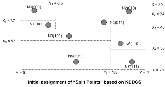
Figure 6: KDDCS original K-D tree
