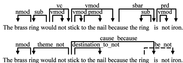
Figure 2. Typical dependency parse revisions to extract reference answer facets
