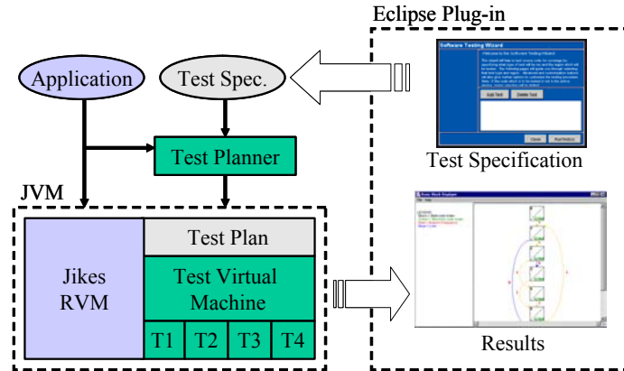
Figure 1: SoftTest testing framework for Java programs
