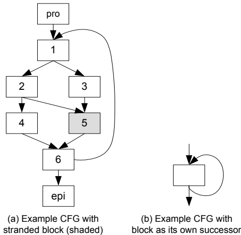
Figure 4: Example CFGs for test planner
