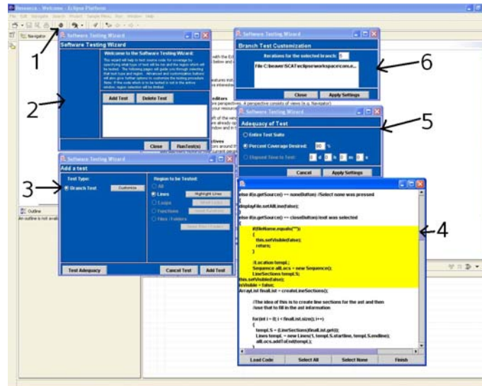
Figure 2: Test specification in Eclipse GUI
