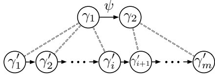
Fig. 3: A graphical representation of semantic lock-step
