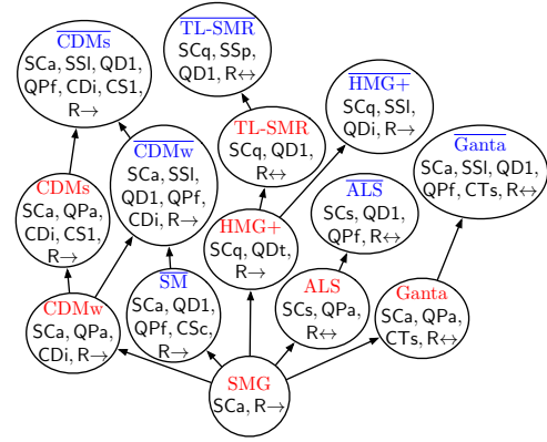
Fig. 6: Partial lattice of canonical usage
