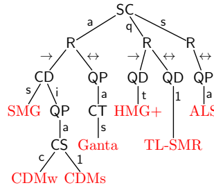
(b) Taxonomy of simulations
