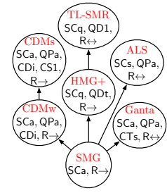
(c) Partial lattice of simulations
