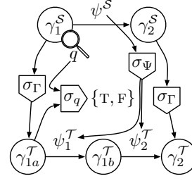
Fig. 1: The general form of an implementable expressiveness mapping.
