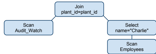
Figure 3: Optimized query tree for Alice's final query.
