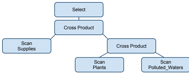
(a) Tree generated by the parsing phase.
