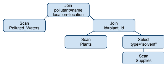
(c) Tree generated by the optimization phase.
