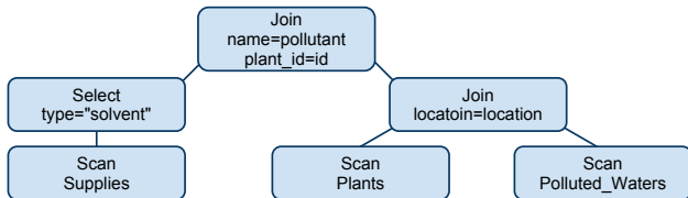
(b) Tree generated by the reorganization phase.
