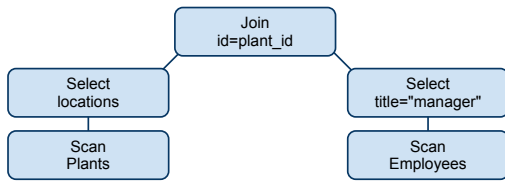
Figure 2: Optimized query tree for Alice's second query.
