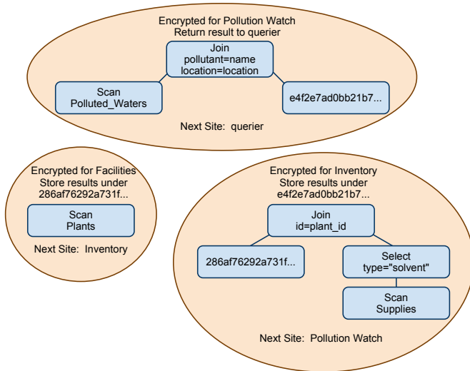
Figure 4: An illustration of a hardened mutant query plan.
