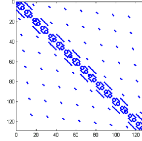
Figure 10. The p -matrix of CG (128 nodes).
