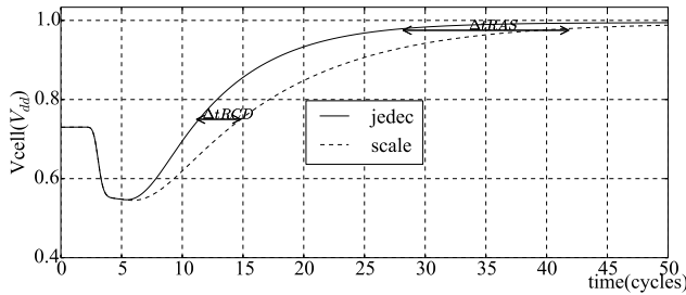
Figure 10: SPICE modeling on \tau_{RCD} and \tau_{RAS} . jedec follows the JEDEC specification and scale meets the projected values. \tau_{RCD} ends at 0.75V_{dd} [46, 34], and \tau_{RAS} completes at 0.975V_{dd} .
