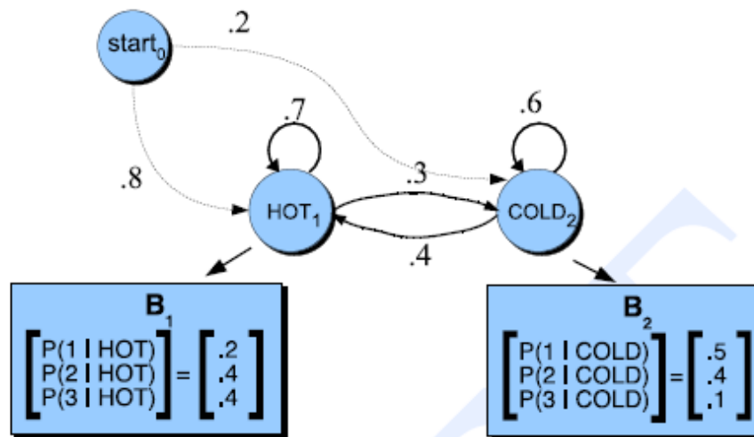
Figure 6.3 A Hidden Markov Model for relating numbers of ice creams eaten by Jason (the observations) to the weather (H or C, the hidden variables). For this example we are not using an end-state, instead allowing both states 1 and 2 to be a final (accepting) state.
